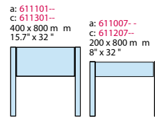
Post and panel Sign Panel: 1 Post: 2/Ø=70 mm / 2.75" Windload A1, A2, B1, B2
