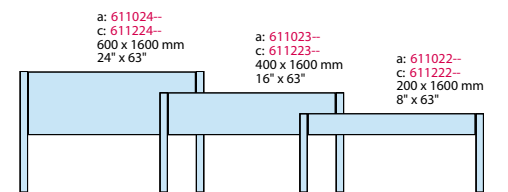
Post and panel Sign Panel: 1 Post: 2/Ø=70 mm / 2.75" Windload A1, A2, B1, B2
