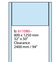
Post and panel Sign Panel: 1 Post: 2/Ø=90 mm / 3.5" Windload A1.
