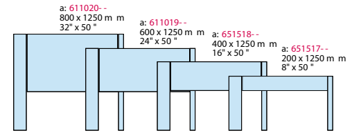
Post and panel Sign Panel: 1 Post: 2/Ø=70 mm / 2.75" & 1/ID 175 mm / 6.875" Windload A1, A2, B1, B2
