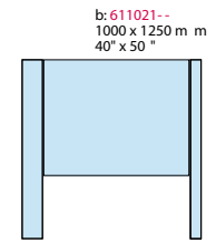
Post and panel Sign Panel: 1 Post: 1/Ø=90 mm / 3.5" & 1/ID 175 mm / 6.875" Windload A1, A2, B1, B2
