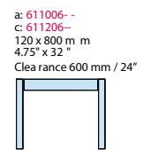
Post and panel Sign Panel: 1 Post: 2/Ø=70 mm / 2.75" Windload A1, A2, B1, B2 Clearance 600 mm / 24"
