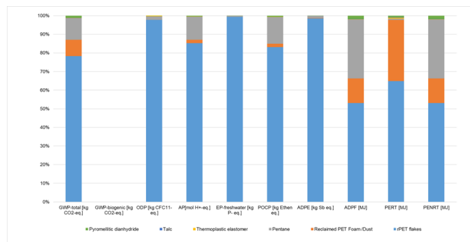
Diagram: Dominance analysis A1 -Raw material acquisition of ArmaPET Eco50
